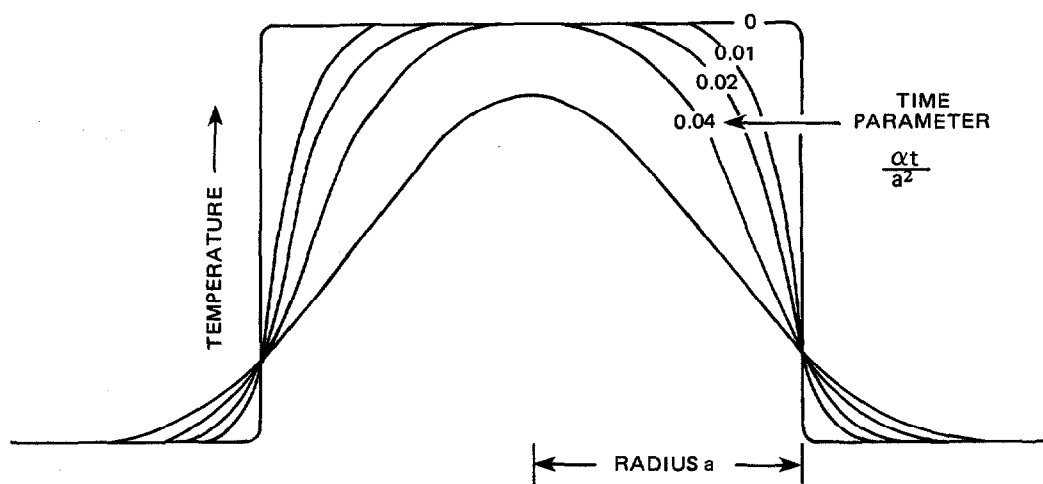
Fig 7 Temperature Distribution During Cooling of a Spherical Element of Inert Material That Has Been Raised Initially to a Uniform Temperature Greater Than That of the Surroundings.
